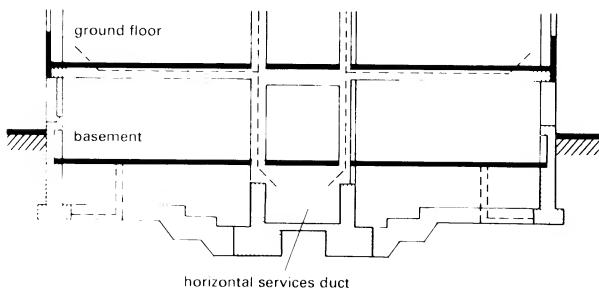
④ Cross-section of lab with well-positioned central corridor
